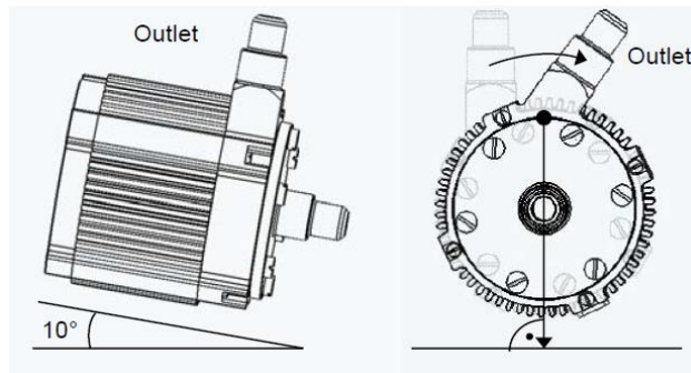
Figure 3: Forward incline (left) / Turned Pump (right)
