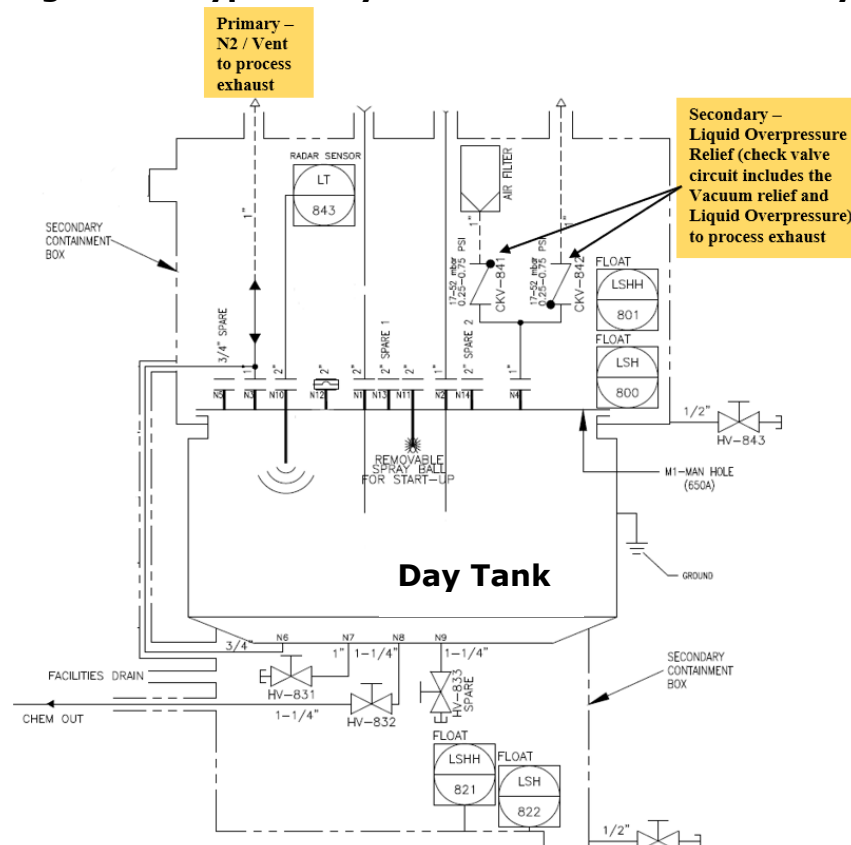
Figure 5 – Typical Day Tank Pressure Protection System Concept
