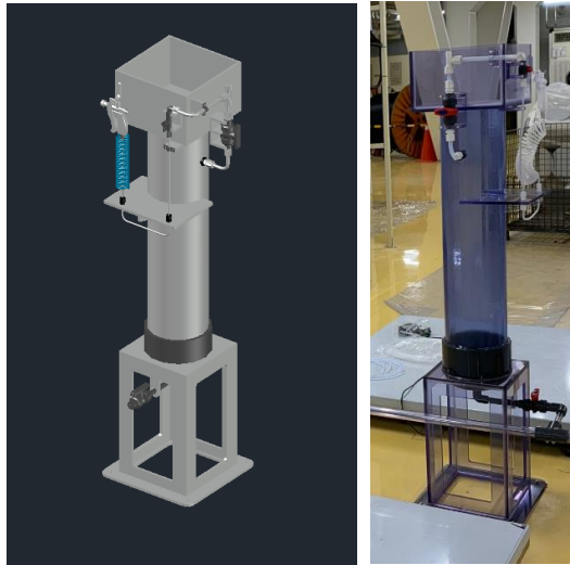
Figure 2 – Slurry Dip tube and Dispense Head Cleaning Module
