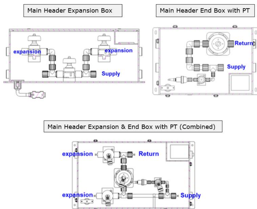
Figure 17 - Different configuration of MHEB and EB
