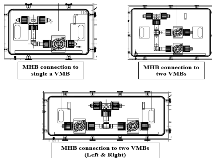
Figure 13 – Different MHB Configurations
