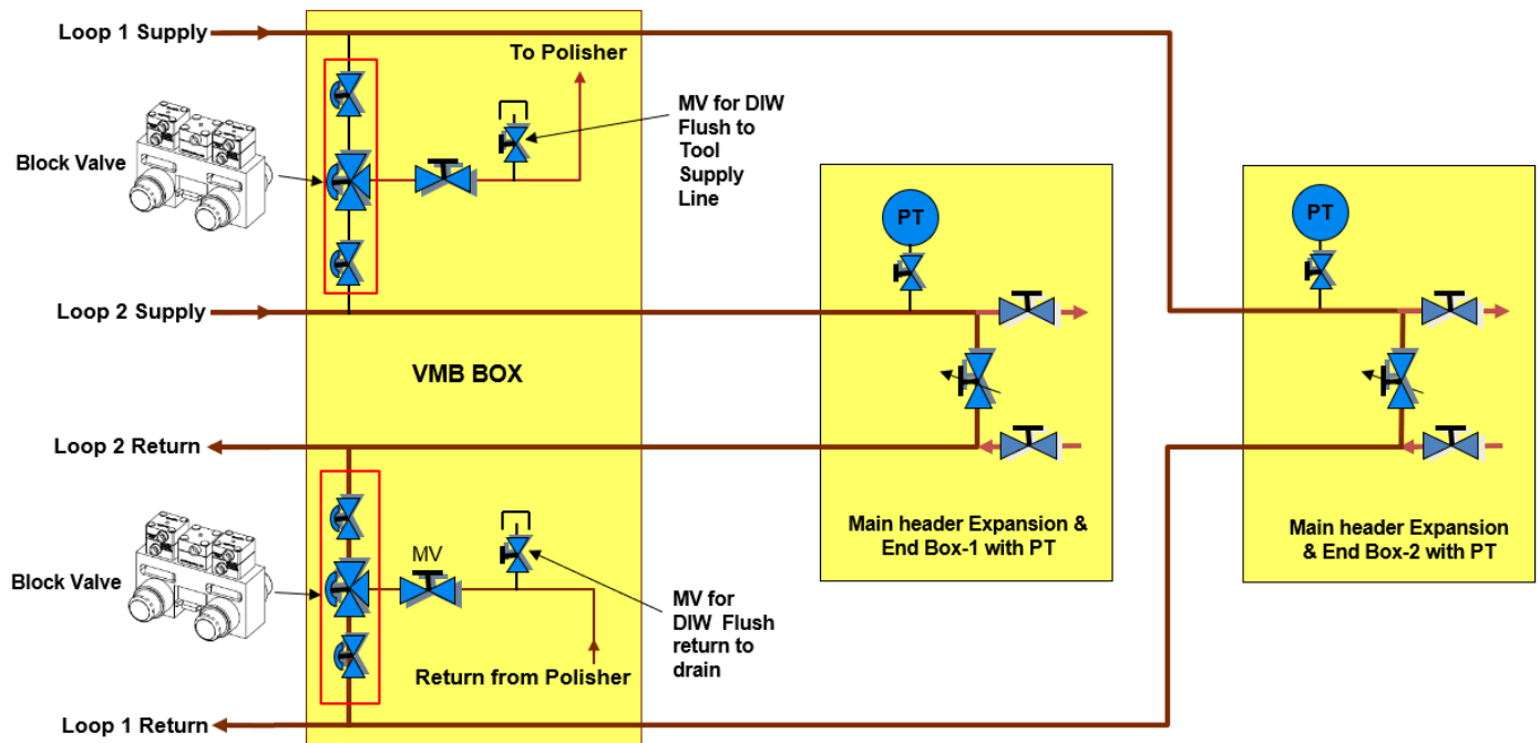
Figure 7 – A Typical Dual Loop VMB with POU Supply/Return and combined MHEB & EB Configuration
