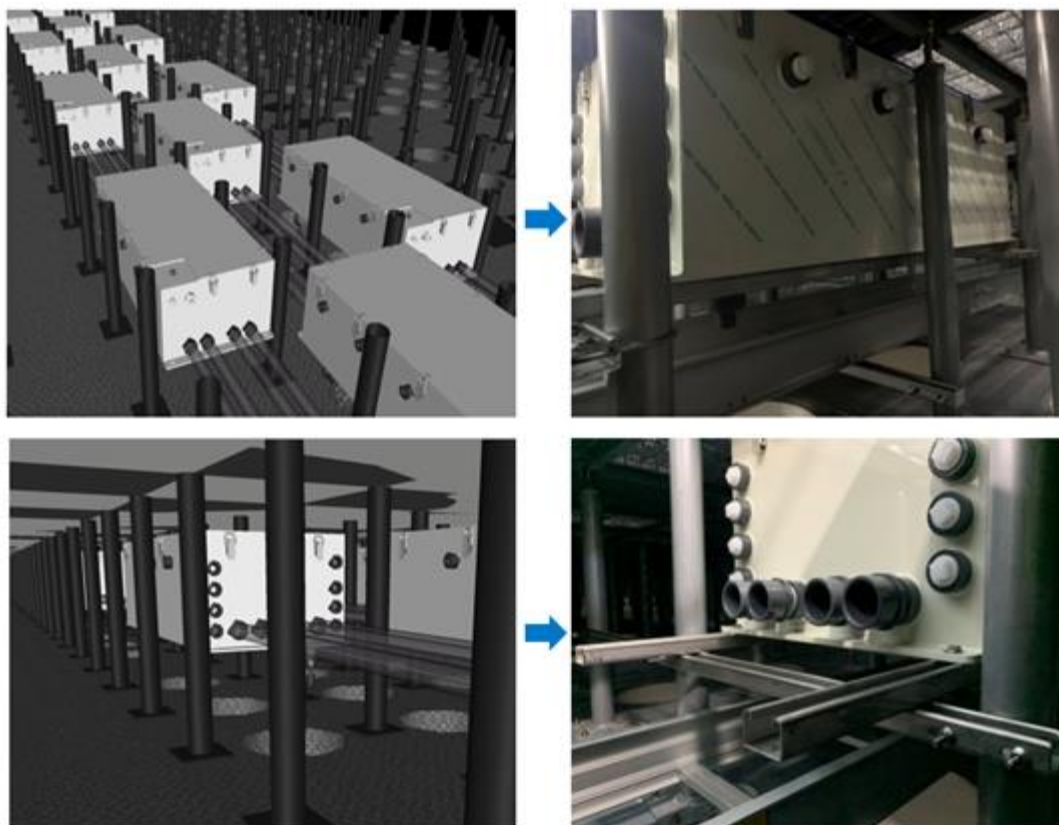
Figure 17 - Different configuration of MHEB and EB
