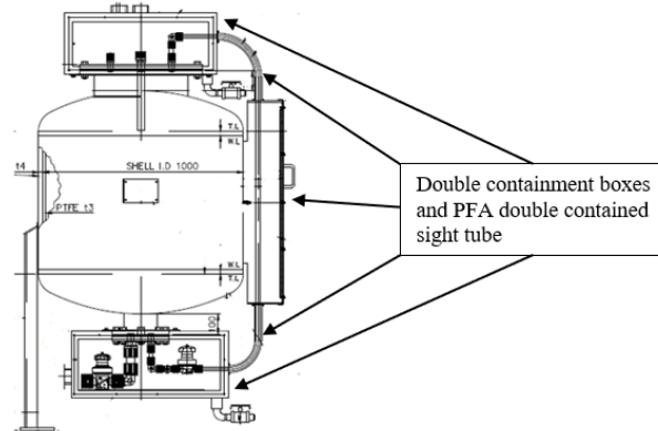
Figure 4 – Typical Tank drawing with containment boxes
