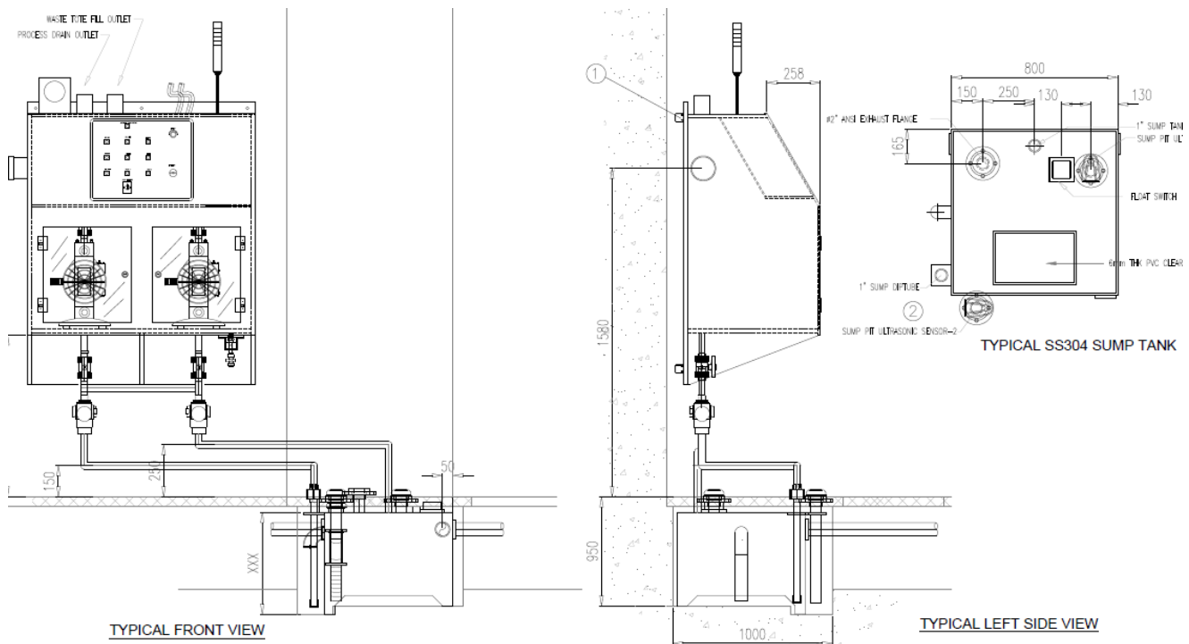
Figure 19 – Typical Dual Sump Pump Lift Station & Pit Tank
