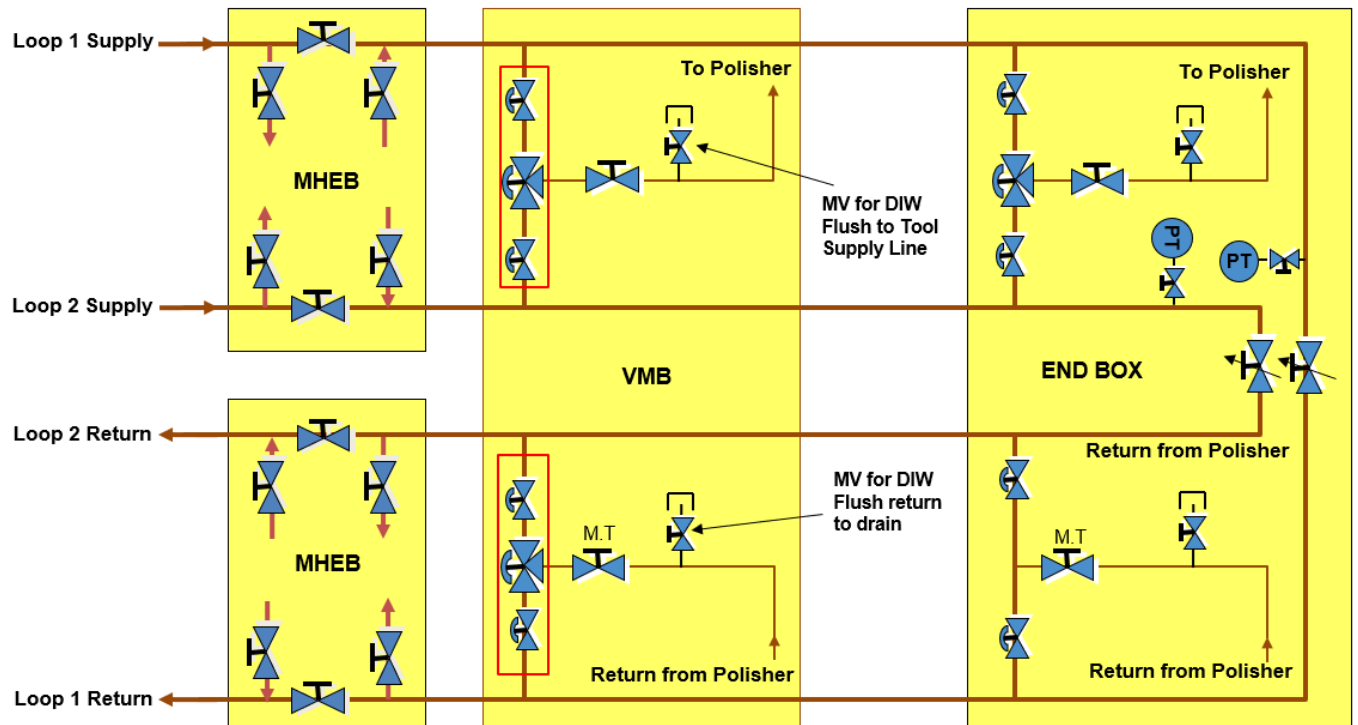
Figure 8 – A Typical Dual Loop VMB with POU Supply/Return with separate MHEB & EB Configuration
