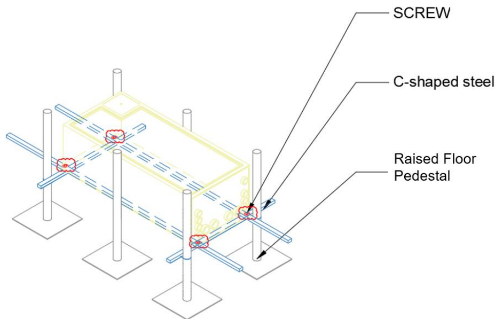
Figure 15 – Flow Through VMB Installation guidelines below Raised Floor in cleanroom
