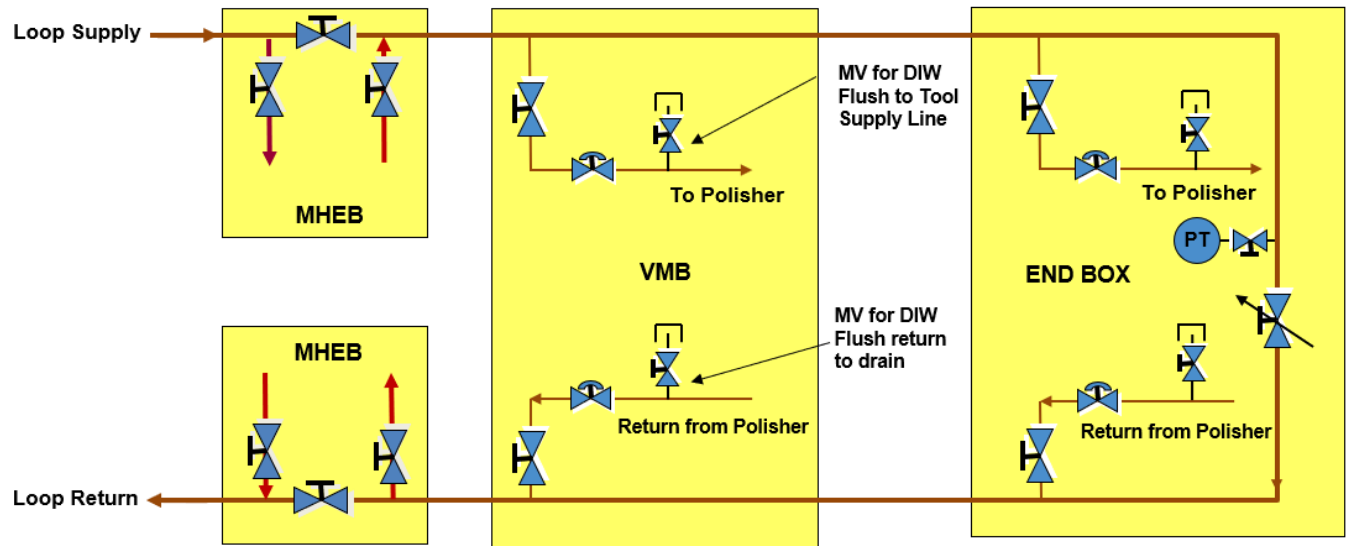
Figure 9 – A Typical Single Loop VMB with POU Supply/Return Configuration
