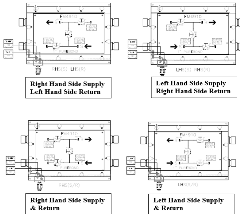
Figure 12 – Different MHEB Typical Configurations
