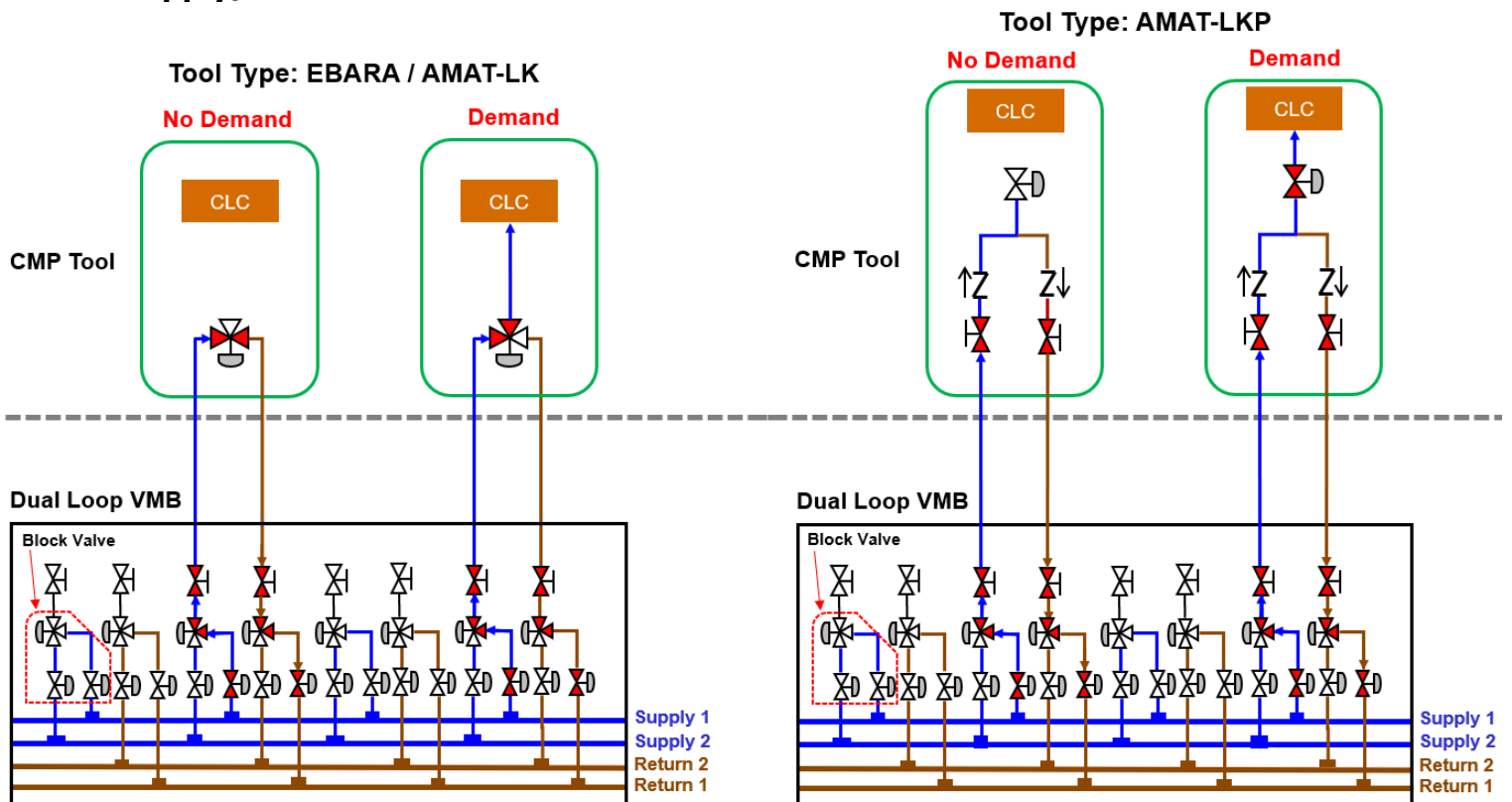
Figure 10 – Typical VMB to CMP Tool configuration for Dual VMB with POU Supply/Return line
