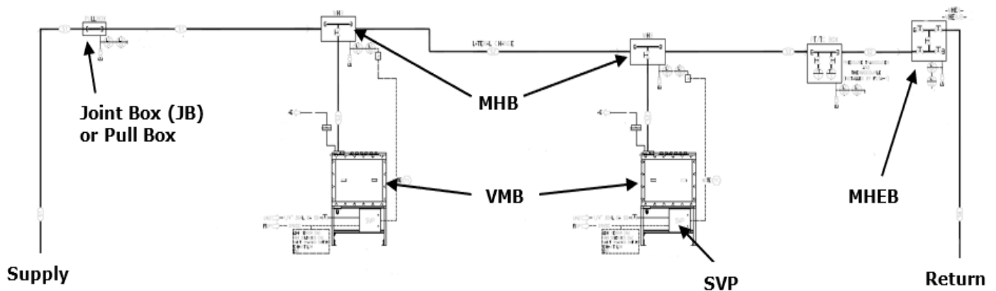
Figure 11 – Typical Main Header Distribution Concept
